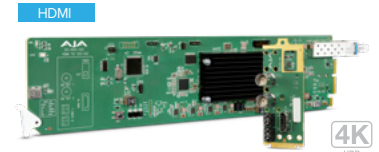
OG-HA5-12G-T-ST $1,435 openGear HDMI 2.0 to 12G-SDI Conversion and ST Fiber Transmitter
